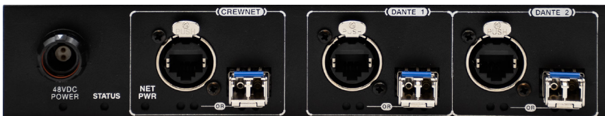
CXD-32CF: Digital Audio Network Interface Rear View
